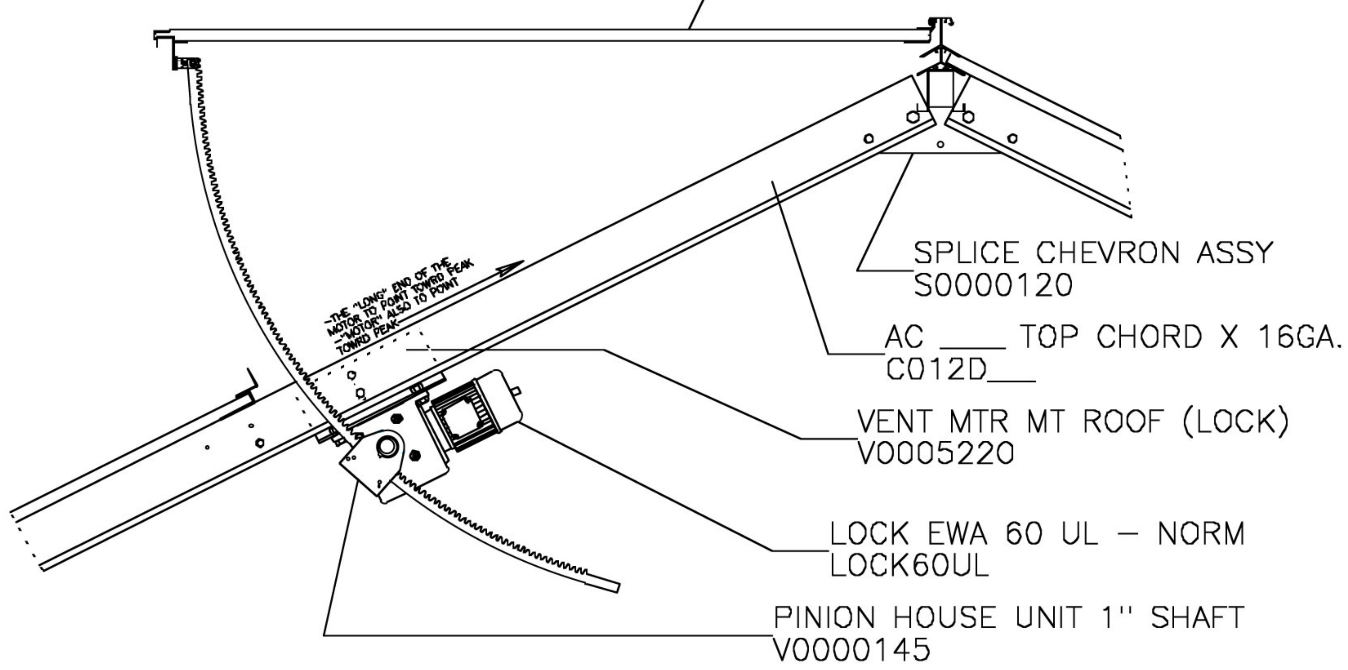
RIDGE VENT ASSEMBLY TYP.
