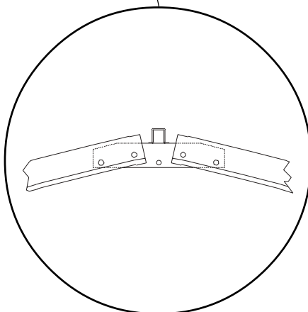
Splice Chevron Joins two arch halves
