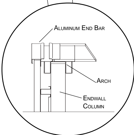
End Bar Trim (OPTIONAL)
